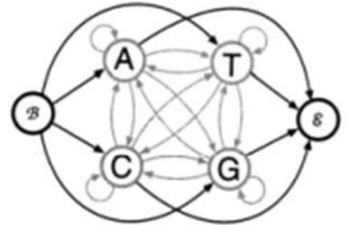
Fig. B. State transition diagram with begin and end states for a Markov model of DNA
